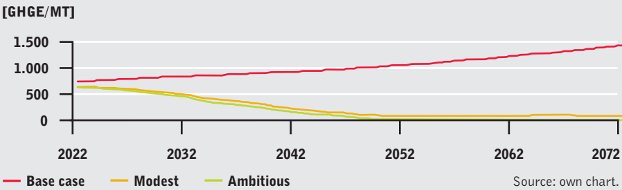
Fig. 2g: Summary of the simulation results Greenhouse gas emissions (MT)
