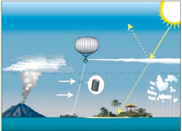
SRM technologies aim to lower the amount of heat in the atmosphere by bouncing sunlight back into space before it becomes trapped in the Earth's atmosphere. Illustration (cc) Hugh Hunt
